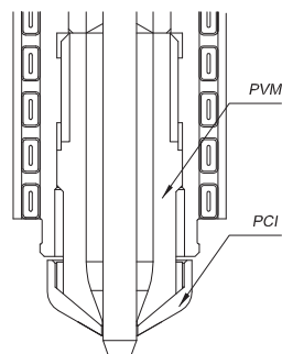
(PHV) Thru Hole Polivalve
