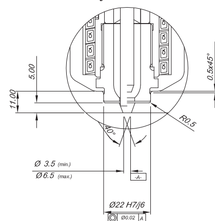
Angular Valve Pin Fit
