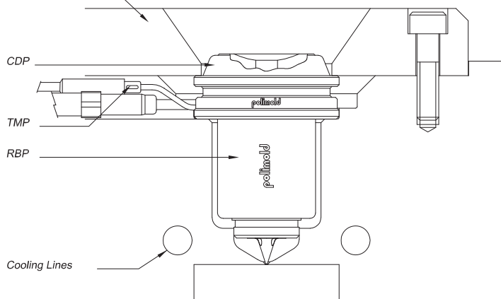
Nozzle Assembly Specification Components
