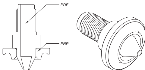
Thru Hole Tip
