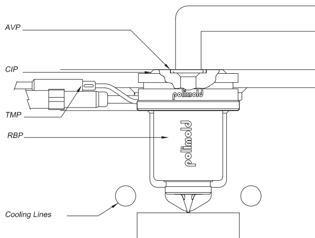
Nozzle Assembly Specification Components
