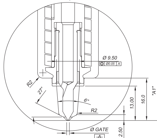
Standard Tip Extended
