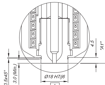
(PMA) Ring Style Tip
