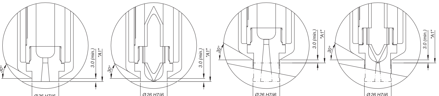
Sprue Tip Extended
