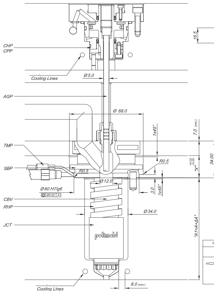
Nozzle Assembly Specification Components
