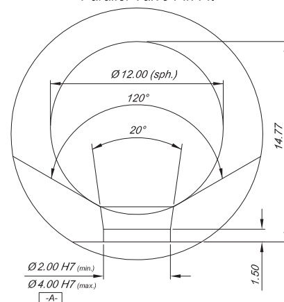
Parallel Valve Pin Fit
