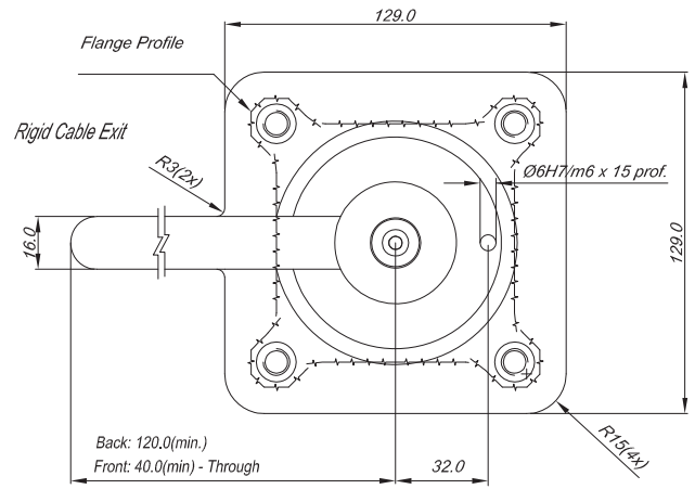
Angular Valve Pin Fit
