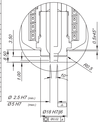
Parallel Valve Pin Fit
