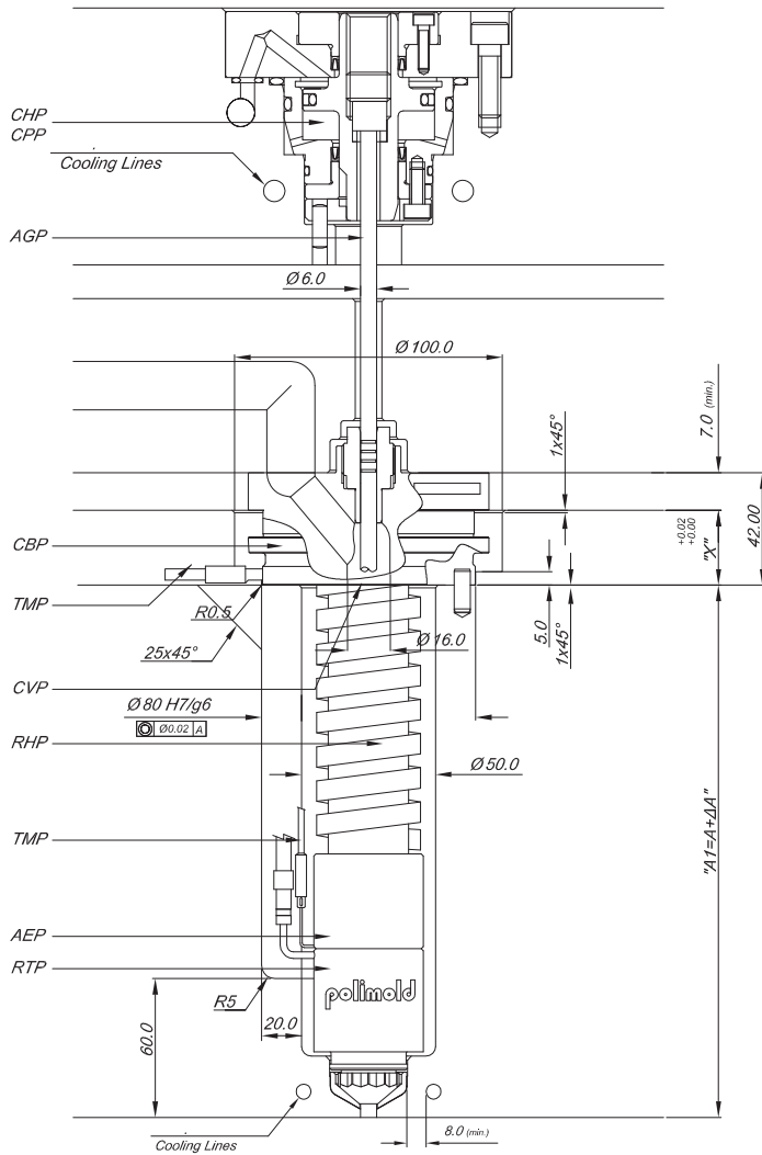
Rigid Cable Exit
