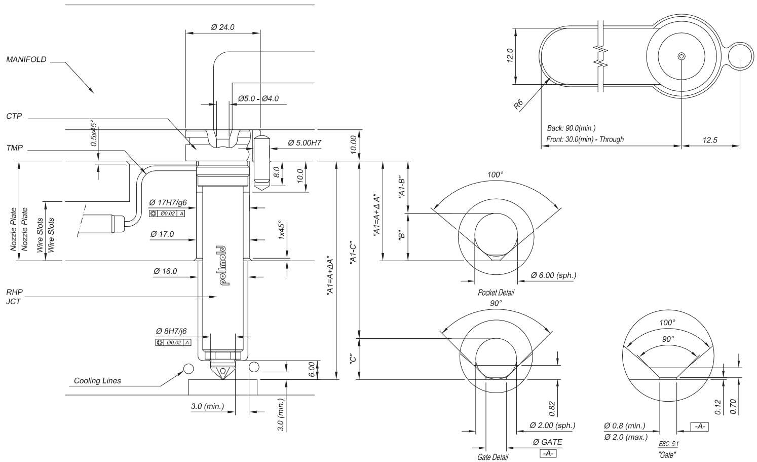
Nozzle Assembly Specification
