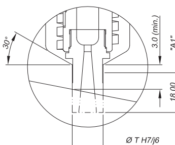
Sprue Tip Extended
