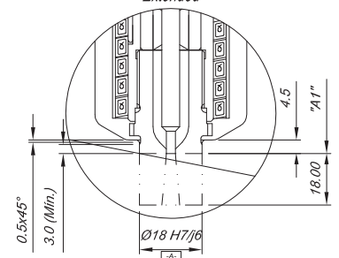
(PMA) Ring Style Tip Extended
