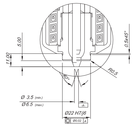
Parallel Valve Pin Fit
