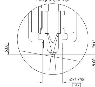
Ring Style Tip
