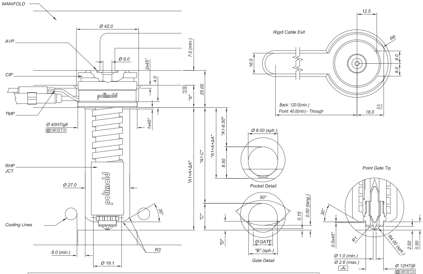
Nozzle Assembly Specification Components
