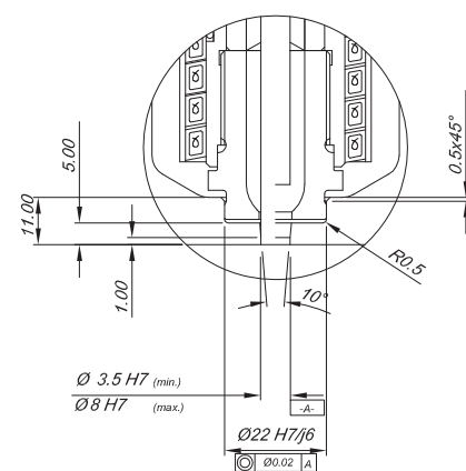
Parallel Valve Pin Fit
