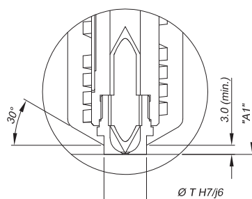
Ring Style Tip
