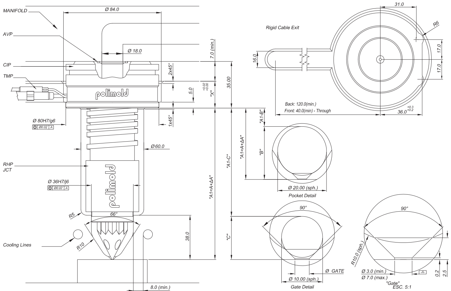
Nozzle Assembly Specification
