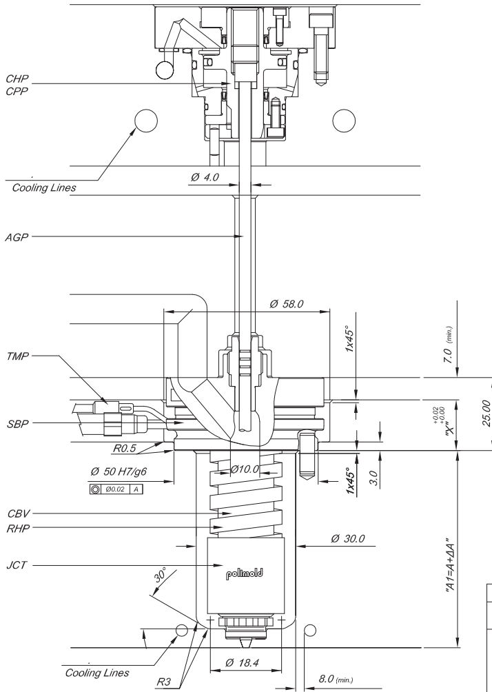
Nozzle Assembly Specification Components
