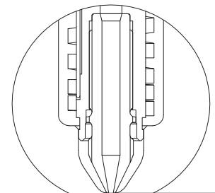
Thru Hole Tip
