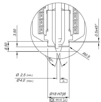
Angular Valve Pin Fit
