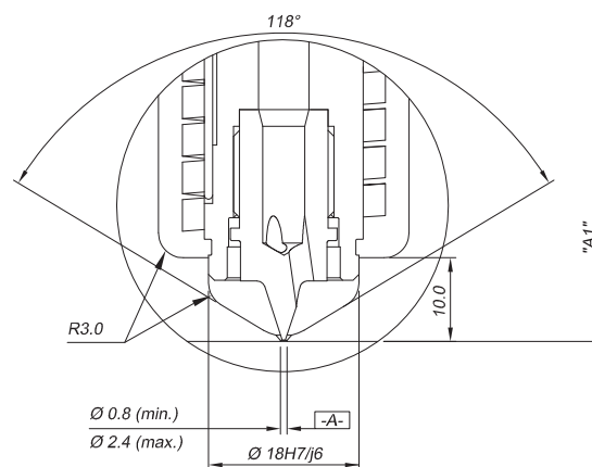
Point Gate Tip
