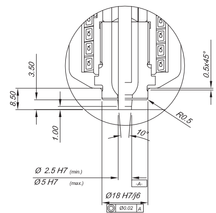
Parallel Valve Pin Fit
