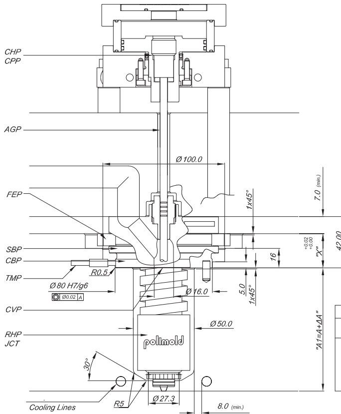
Nozzle Assembly Specification Components
