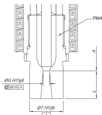
(PMA) Ring Style Tip Extended Angular Valve Pin Fit
