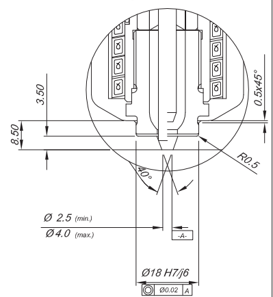
Angular Valve Pin Fit
