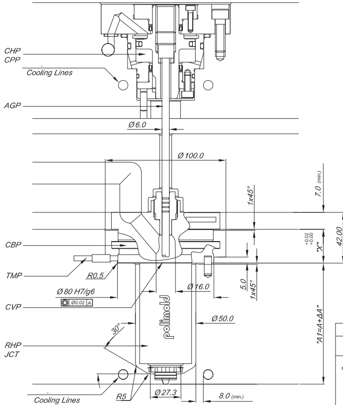
Rigid Cable Exit
