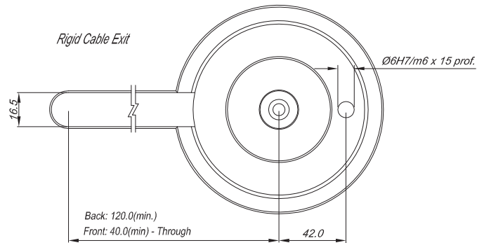
Angular Valve Pin Fit
