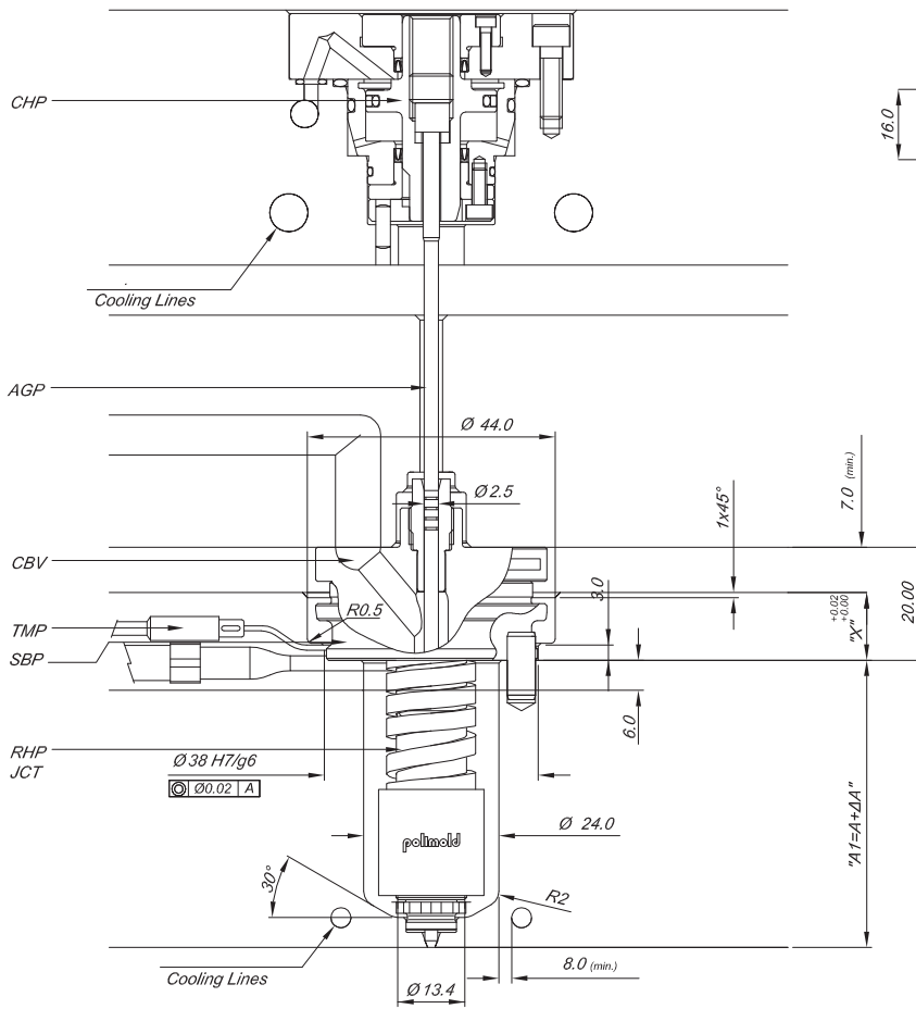
Nozzle Assembly Specification Components
