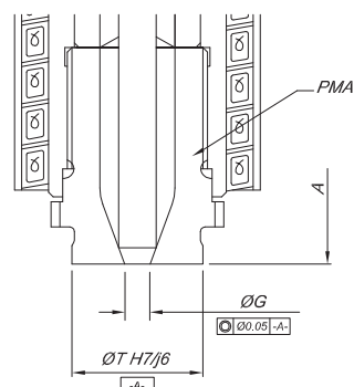
(PMA) Ring Style Tip Angular Valve Pin Fit
