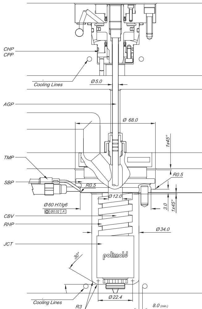
Nozzle Assembly Specification Components
