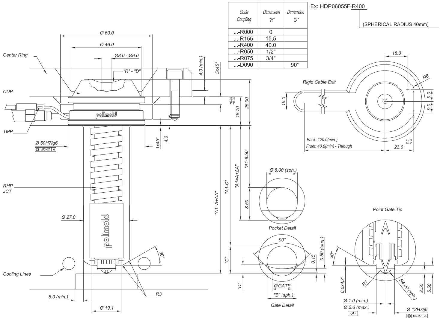
Nozzle Assembly Specification Components
