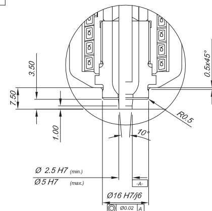
Code Nozzle Dimension "A" Components Tips PVM Tips PMA Body Shoulder Flange Heater Wattage Thermocouple Heater Cables Assembly Option Back BVE12058-D 58.00 54.00 CBV12053-D SBP12022-D FEP12010-D RBP10056 500W TMP01080 BVE12070-D 70.50 66.50 RBP10069 690W TMP01100 BVE12083-D 83.00 79.00 RBP10081 760W TMP01120 BVE12095-D 95.50 91.50 RBP10094 760W TMP01140 BVE12108-D 108.00 104.00 RBP10107 760W TMP01160 BVE12133-D 133.00 129.00 RBP10131 850W TMP01180 Front BVE12159-D 159.00 155.00 RBP10158 1100W TMP01200 BVE12185-D 185.00 181.00 RBP10183 1300W TMP01220 BVE12058F-D 58.00 54.00 RBP10056F 500W TMP01080 BVE12070F-D 70.50 66.50 RBP10069F 690W TMP01100 BVE12083F-D 83.00 79.00 RBP10081F 760W TMP01120 BVE12095F-D 95.50 91.50 RBP10094F 760W TMP01140 BVE12108F-D 108.00 104.00 RBP10107F 760W TMP01160 BVE12133F-D 133.00 129.00 RBP10131F 850W TMP01180 BVE12159F-D 159.00 155.00 RBP10158F 1100W TMP01200 BVE12185F-D 185.00 181.00 RBP10183F 1300W TMP01220
