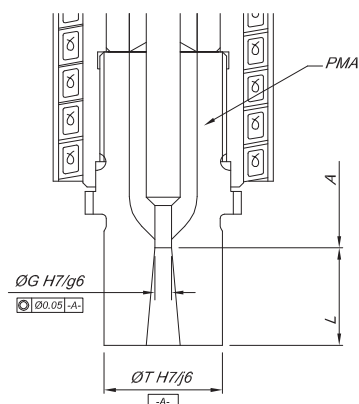
(PMA) Ring Style Tip Extended Parallel Valve Pin Fit
