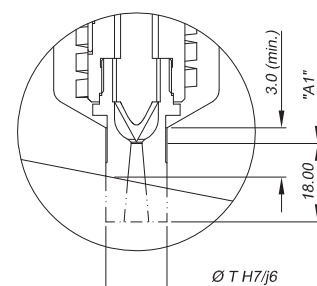
Ring Style Tip Extended
