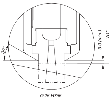
Sprue Tip Extended
