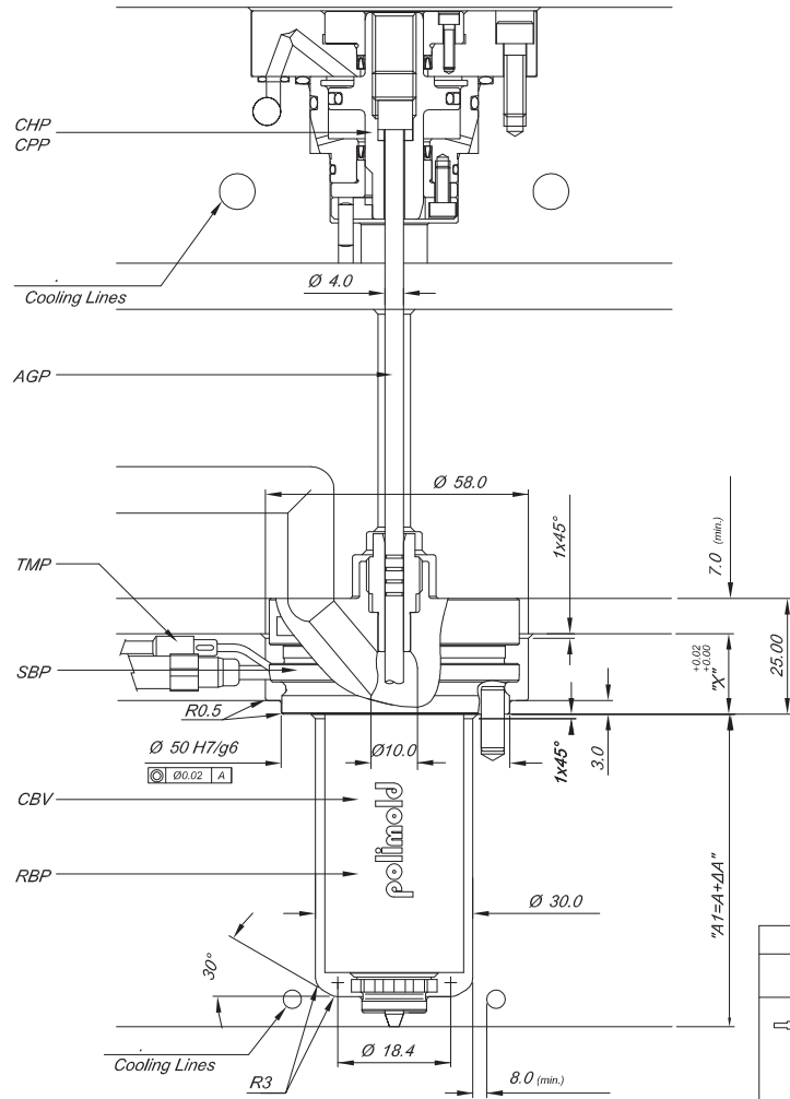
Nozzle Assembly Specification Components
