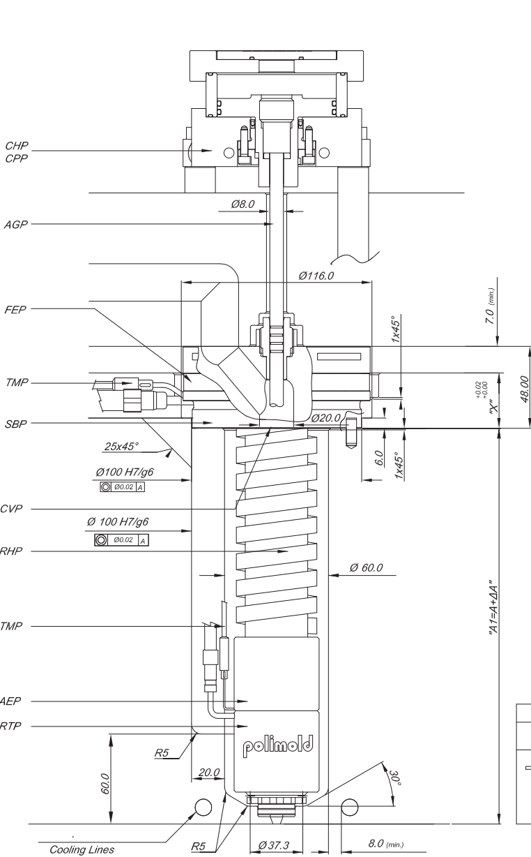
Nozzle Assembly Specification Components
