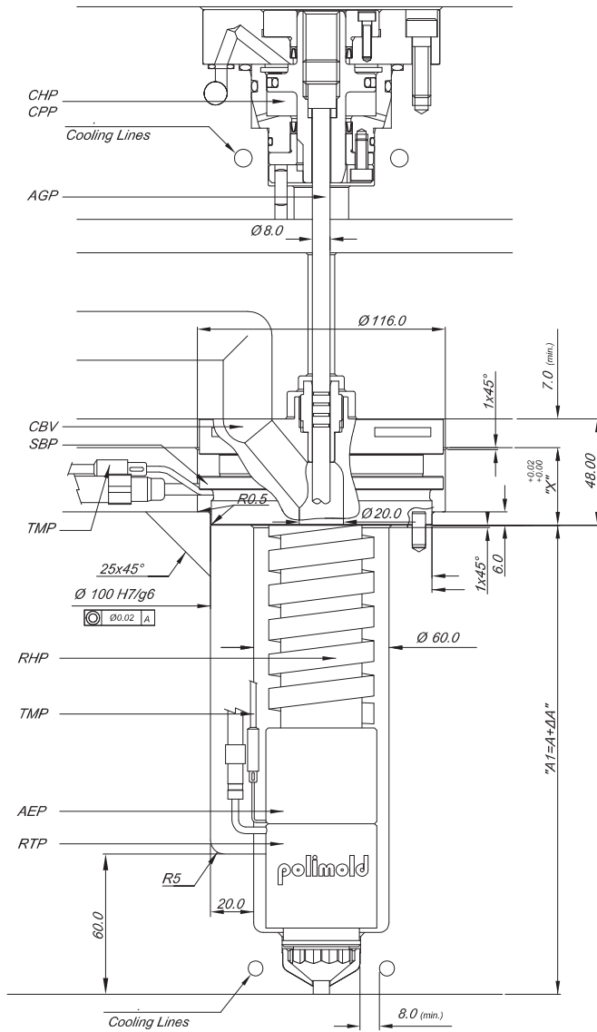
Nozzle Assembly Specification Components
