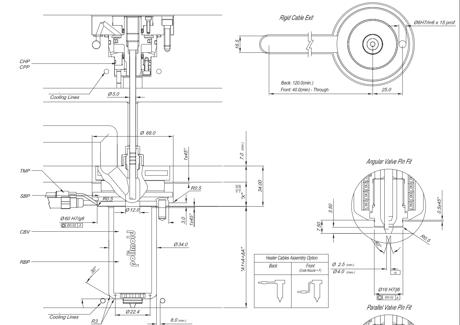
Nozzle Assembly Specification Components
