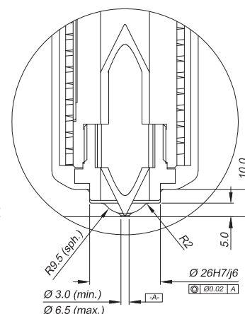
Point Gate Tip
