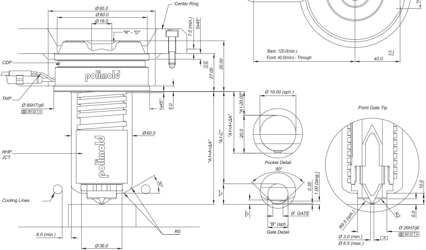
Nozzle Assembly Specification
