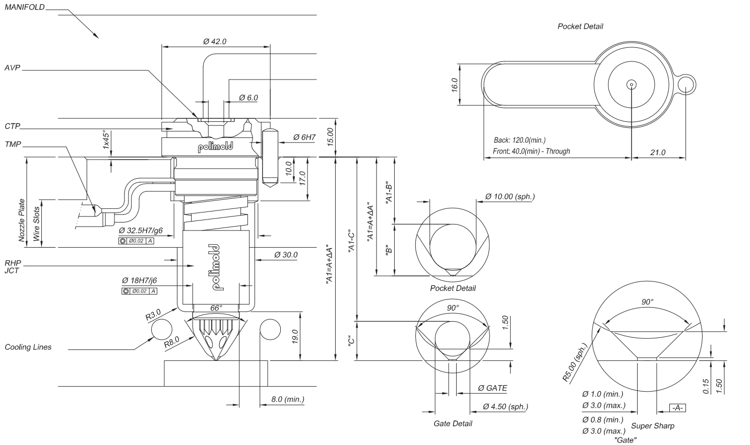
Nozzle Assembly Specification Components
