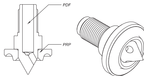
Point Gate Tip
