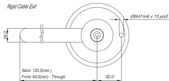
Angular Valve Pin Fit
