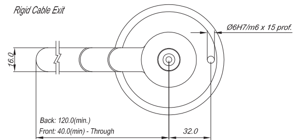
Angular Valve Pin Fit
