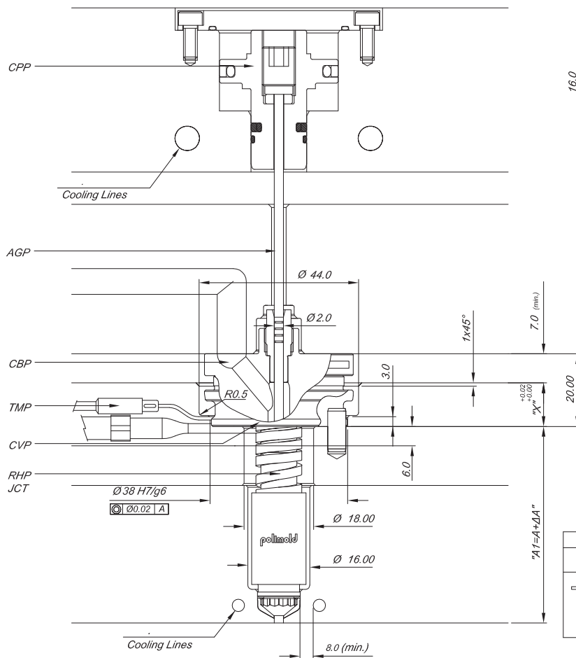
Nozzle Assembly Specification Components
