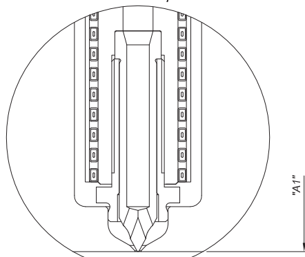
Standard Tip
