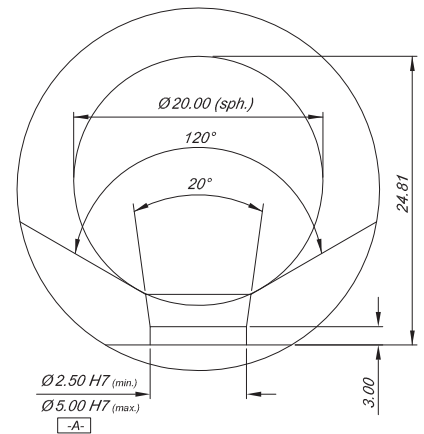
Parallel Valve Pin Fit
