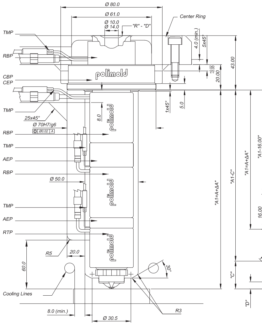
Nozzle Assembly Specification
