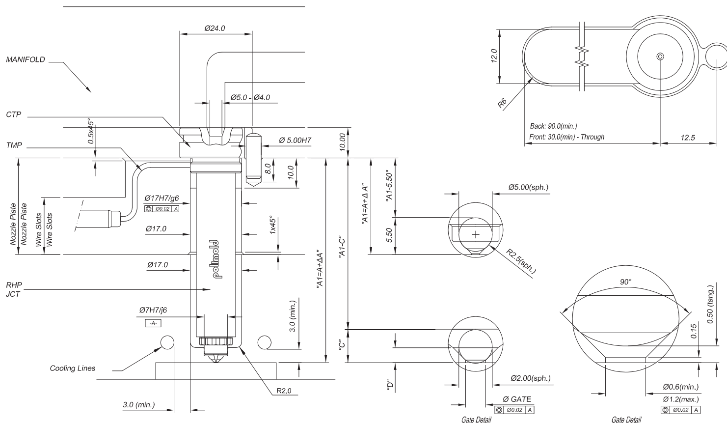
Nozzle Assembly Specification
