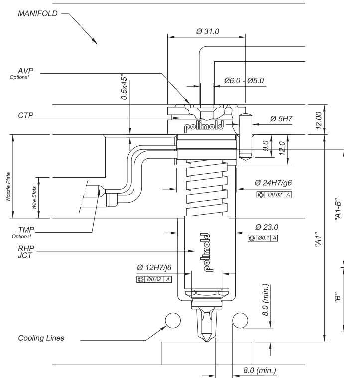
Nozzle Assembly Specification
