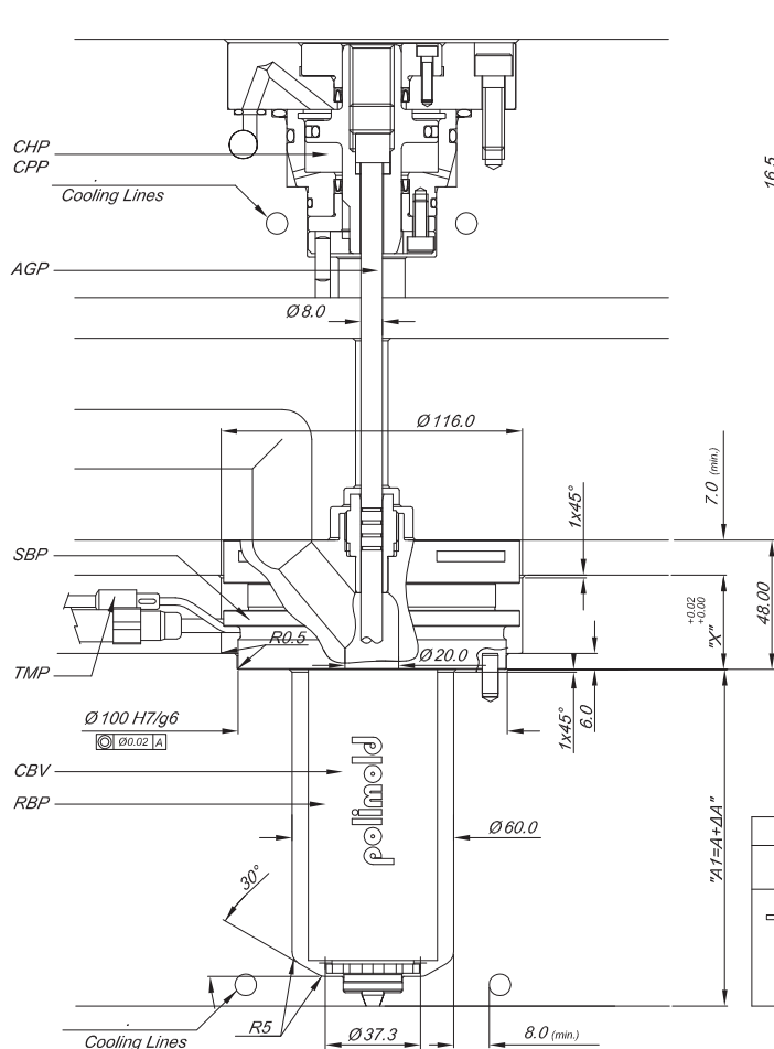
Rigid Cable Exit
