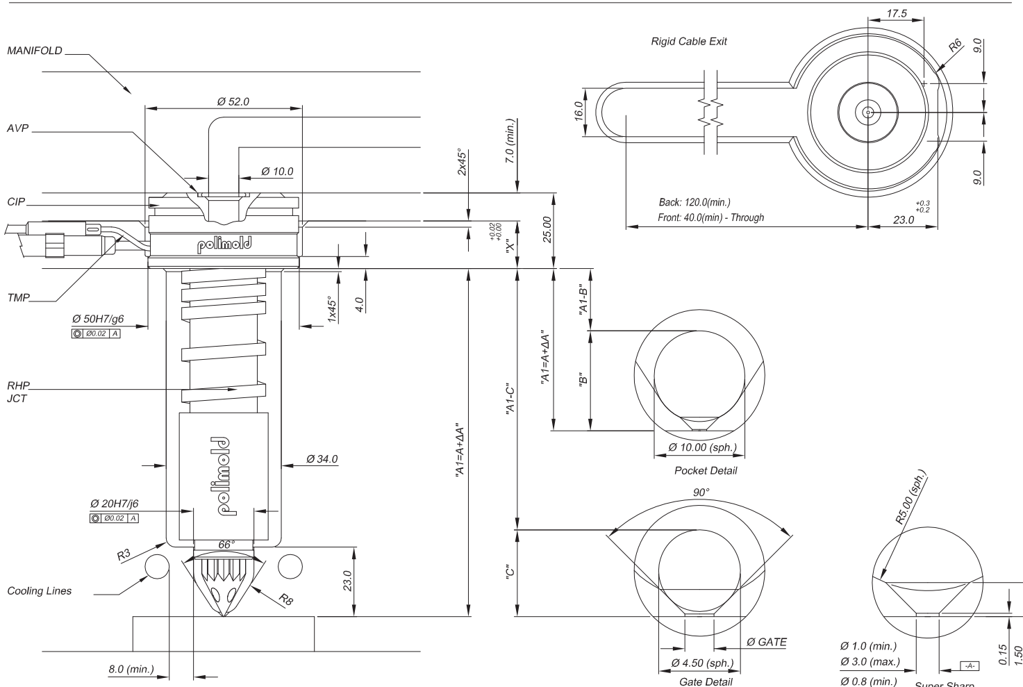
Nozzle Assembly Specification
