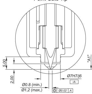
Point Gate Tip
