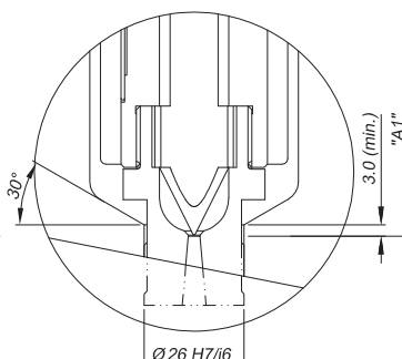
Ring Style Tip Extended
