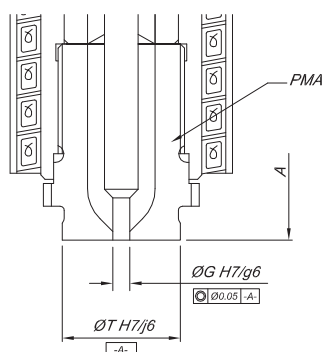
(PMA) Ring Style Tip Parallel Valve Pin Fit
