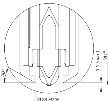
Ring Style Tip
