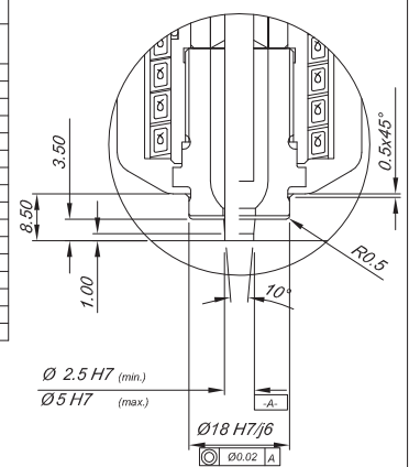
Parallel Valve Pin Fit
